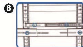
Now put the center slide right next to the rackmount chassis. You should be able to find screw holes on both sides of chassis. Holes are used for mounting the center slide. Later the center slide will be use for attaching the sliding rail.
